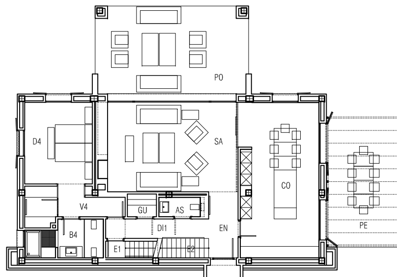
PLANTA BAJA / GROUND FLOOR 1 / 200
