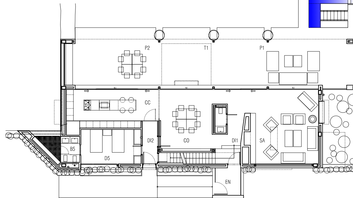
PLANTA BAJA / GROUND FLOOR 1 / 200
